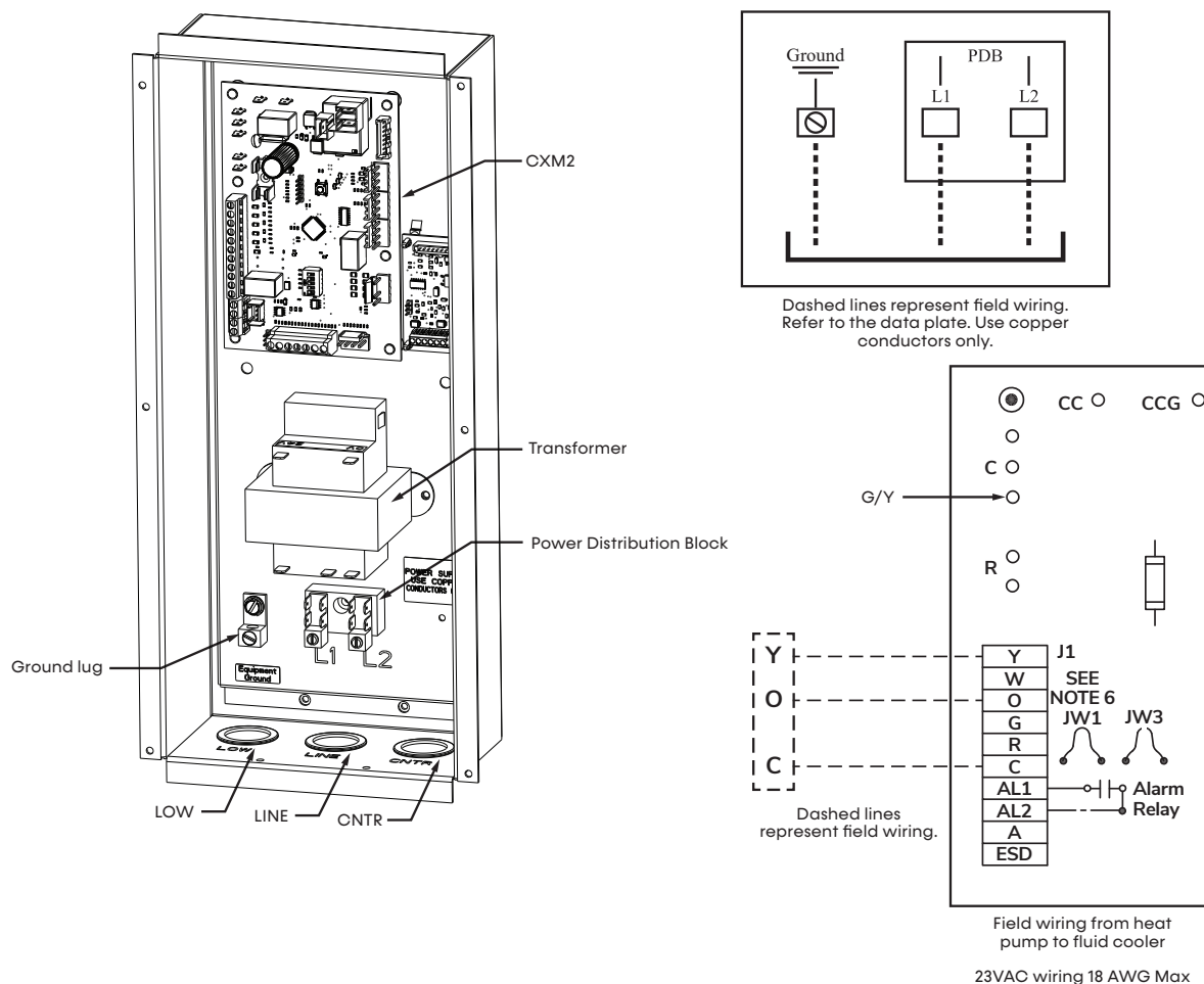
Figure 1: TFC Control Field Wiring
